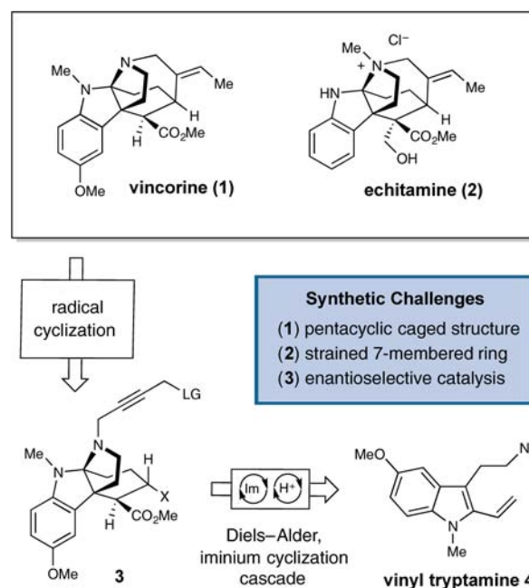
Scheme 1. Akuammiline Alkaloids—Retrosynthesis of Vincorine
